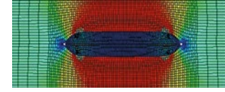
Finite Element Analysis (FEA) model. Red indicates optimal sealing stress.
