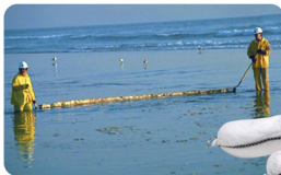
These two men are cleaning a marine spill with numerous booms linked together by their end rings
